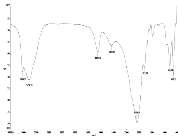
Figure 3.1: FTIR spectrum of bentonite clay.
