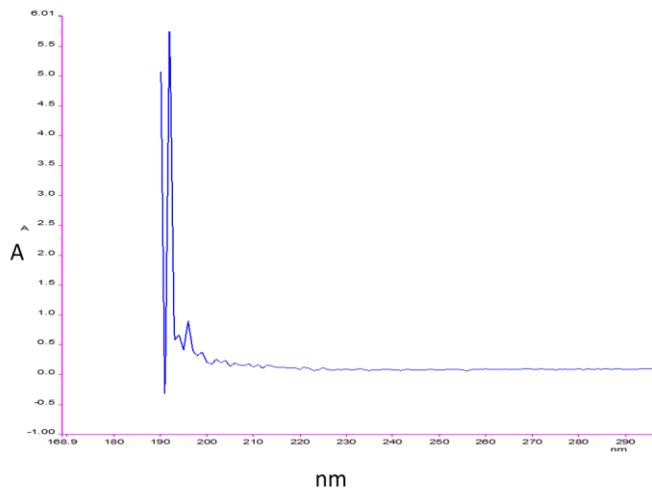
Figure 3.4: Solid state UV-VIS spectrum of organo-nanoclay.
