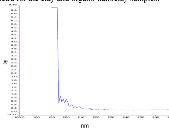
Figure 3.3: Solid state UV-VIS spectrum of bentonite clay.
