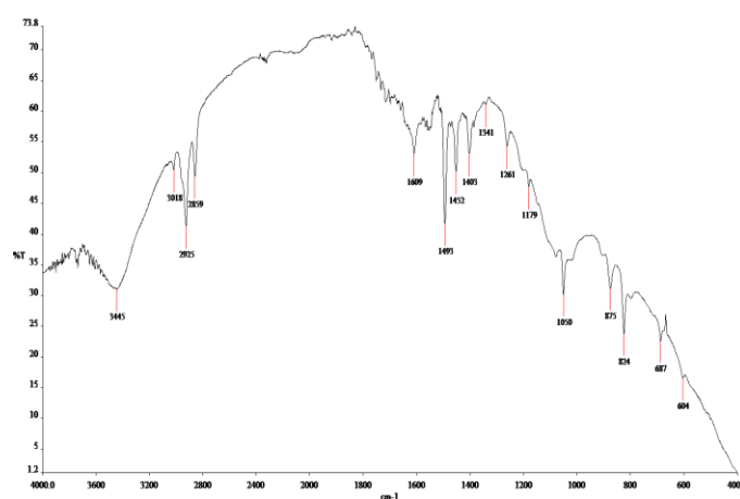
Figure 3.2: FTIR spectrum of organo-nanoclay.
