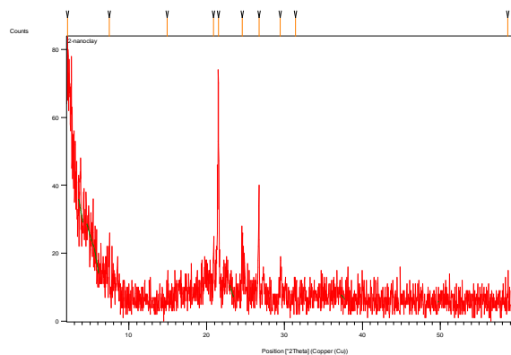
Figure 3.7: X-ray diffraction pattern of organo-nanoclay.
