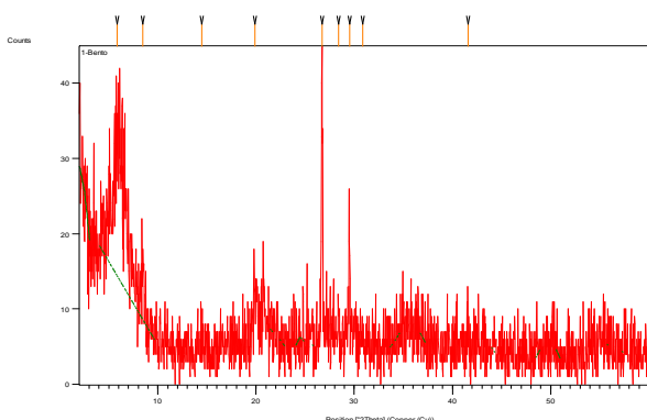
Figure 3.6: X-ray diffraction pattern of bentonite clay.
