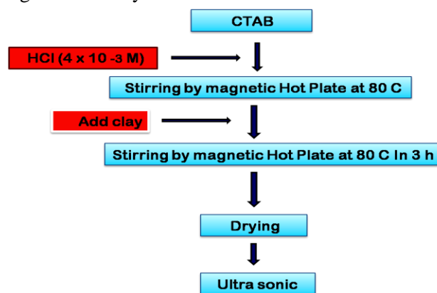
Figure 2.1 schematic synthesis of organo-nanoclay.
