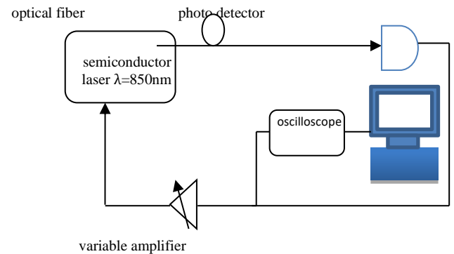
Sketch of the experimental setup of a semiconductor
