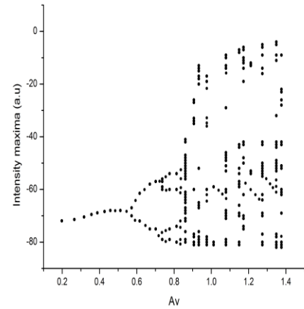
Fig. 4 : bifurcation diagram for the variation of feedback strength
