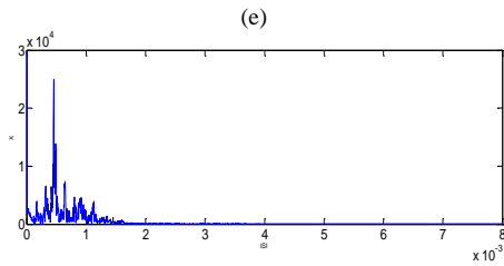
Fig. 2: Experimental time series at bias current values(a)3mA,(b)14mA,(c) the corresponding power spectrum at14mA, ( (d)the corresponding attractor at 14mA, ,(e) inter spike interval (ISI)at 14mA.
