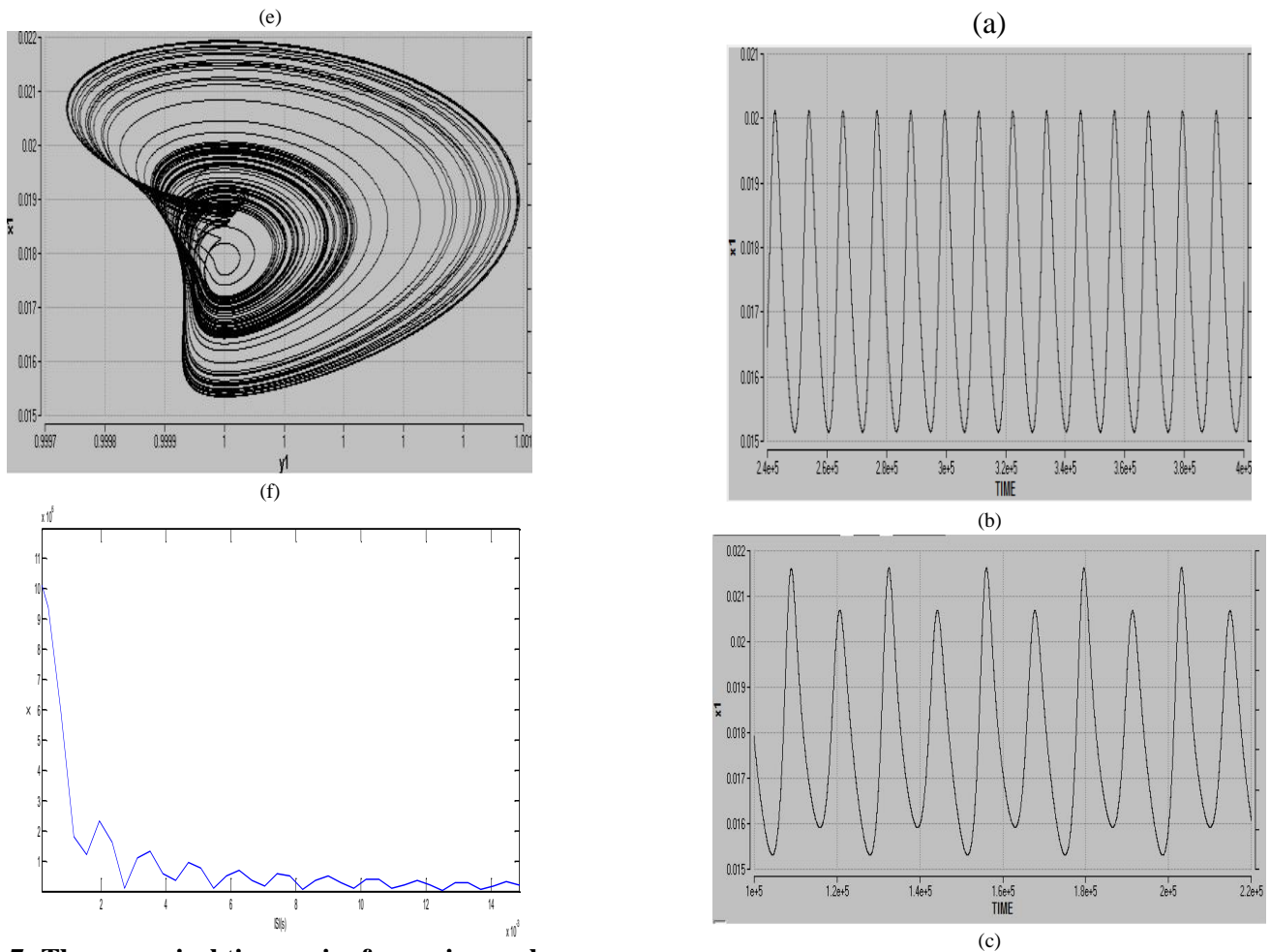
Fig.7: The numerical time series for various values of feedback strength (a)0.988,(b)0.992,(c)0.997,(d)FFT at the chaotic state,(e) the corresponding attractor of the chaotic state(0.997),(f) ISI at the chaotic state.
