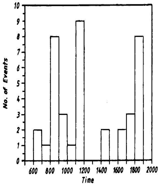
Figure (2) Temporal Distribution of the SCR Seismicity in the Arabian Plate.
