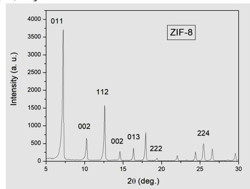
Fig.2 XRD of ZIF-8 on pores \text{Al}_2\text{O}_3
