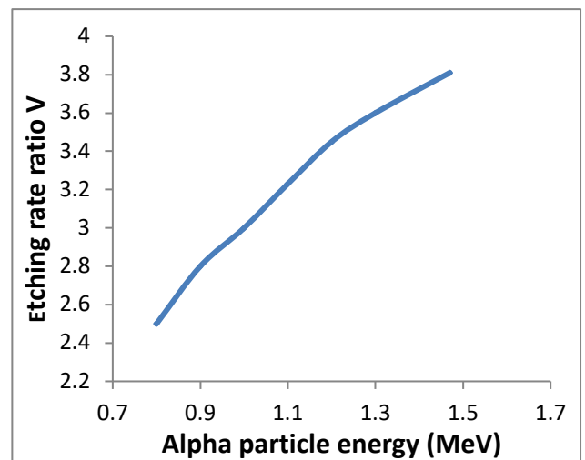
Figure. 6. etch rate ratio as a function of the alpha particles with different energies in the CR-39 nuclear track detector and etched in 6.25N NaOH at 70±1 °C.
