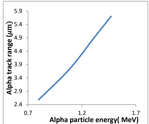
Figure. 5. Alpha particle range as a function of the different energies in the CR-39 nuclear track detector and etched in 6.25N NaOH at 70±1 °C.
