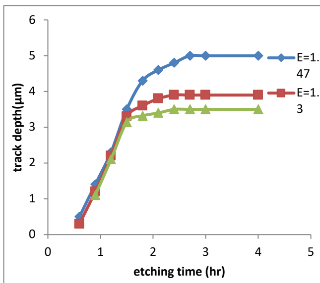
Figure.4.shows the depth of the alpha particle path within the detector material as a function of the different etching time for the different energies of the particle with etchant solution of 6.25N NaOH at 70±1 °C.
