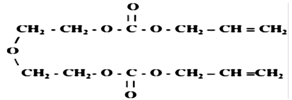
Figure. 1. A periodical monomer unity constructure in the CR-39 detector. [4].
